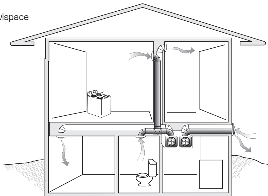
Figure 9.4: Balanced non-heat-recovery ventilation. (Only a few manufacturers provide balanced ventilators without heat recovery.)
