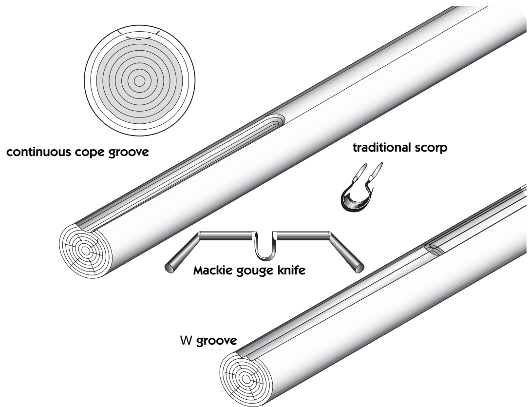
A sequence for cutting the W groove
