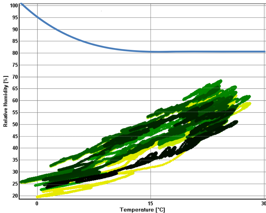
Figure 17. Modeled isopleths showing the distribution of temperature and RH at exterior side of air barrier system.
