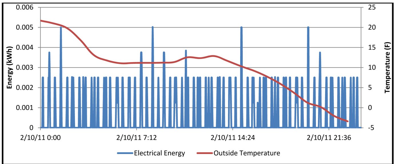
Figure 12. The energy use of the Sun Frost passive prototype on a warmer day. The average outside temperature on Feb. 10, 2011 was 13^{\circ}\text{F} .
