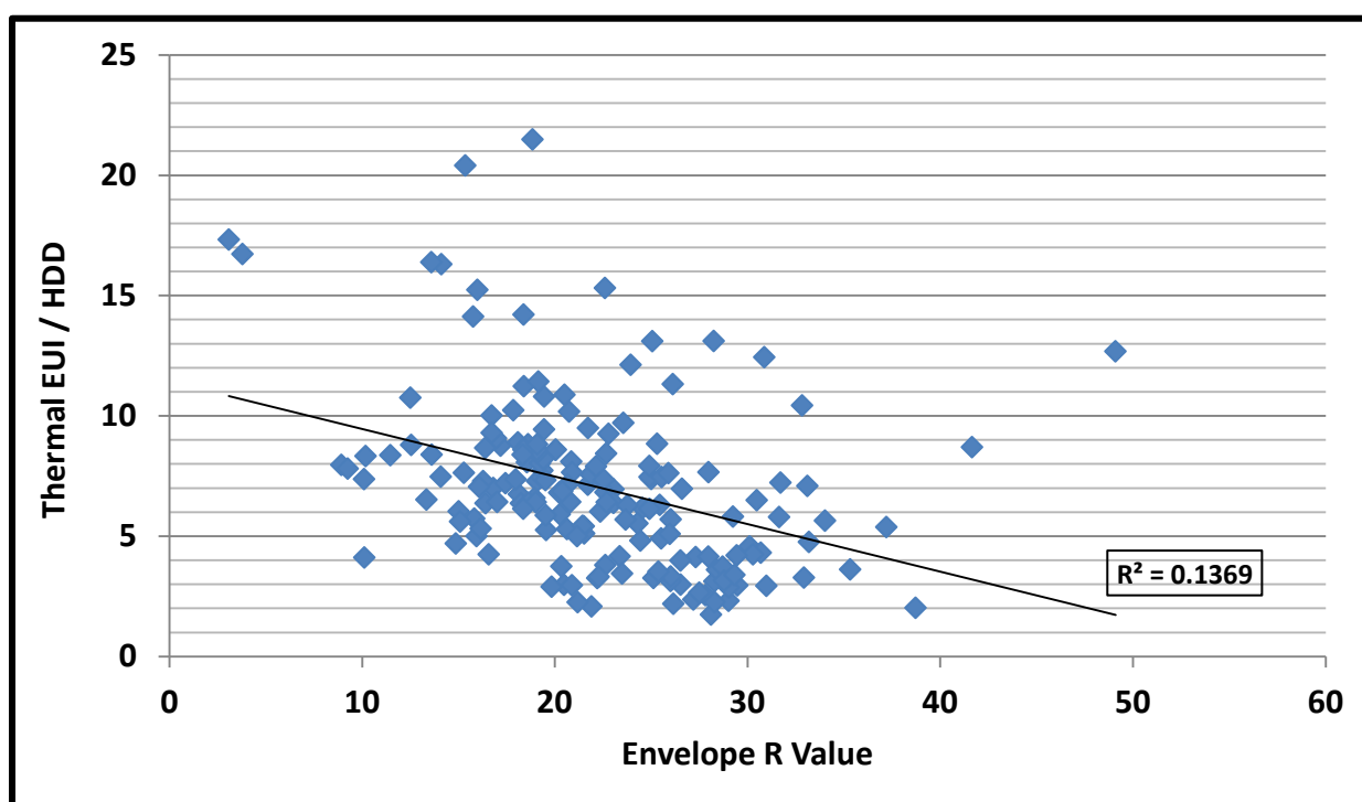
Figure 32: Schools - Thermal EUI/HDD vs. Envelope R-value A
