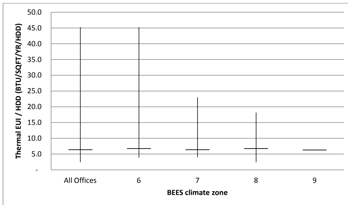
Figure 44: Median Thermal EUI/HDD by Climate Zone for Offices A
