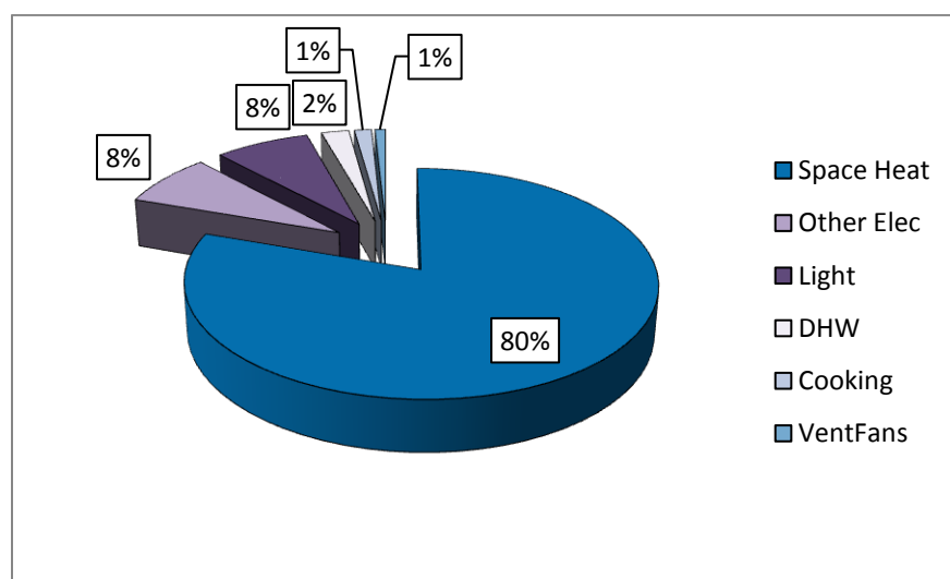
Figure 51: Maintenance / Shop - Energy Consumption by End Use A
