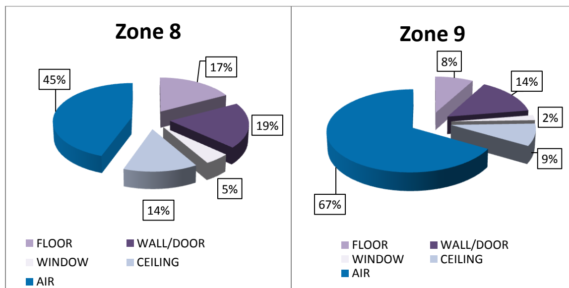
Figure 15: Heat Loss by Component - Climate Zones 8 and 9A
