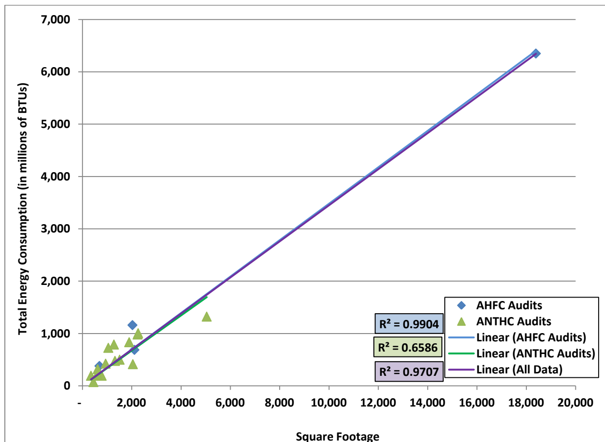
Figure J: Comparison of Washateria and Water Plant AHFC and ANTHC Audit Data
