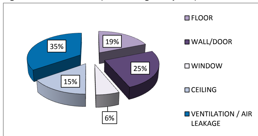
Figure 71: Health Clinic - Space heating loss by component A
