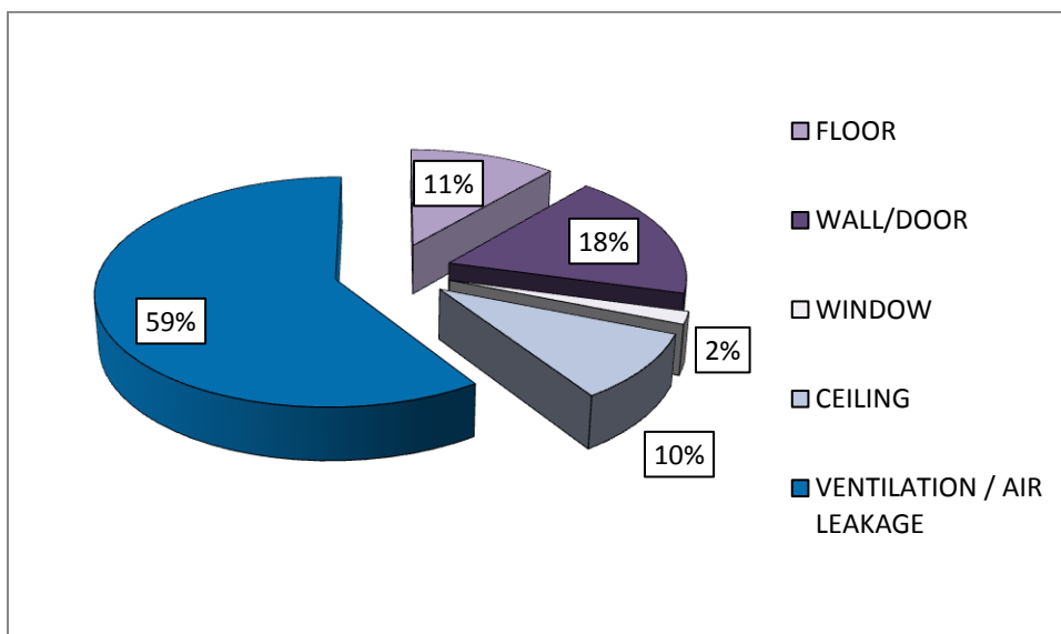
Figure 74: Athletic Facilities - Space heat loss by component A
