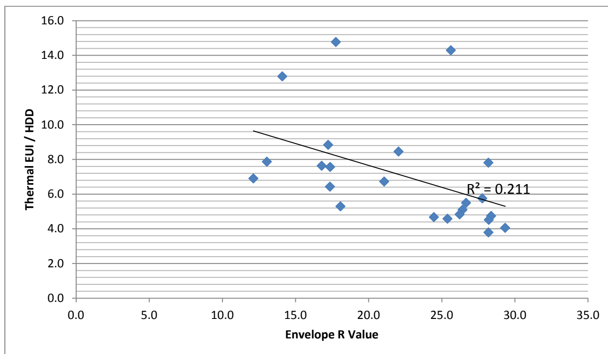
Figure 72: Health Clinic - Thermal EUI/HDD vs. Envelope R-value
