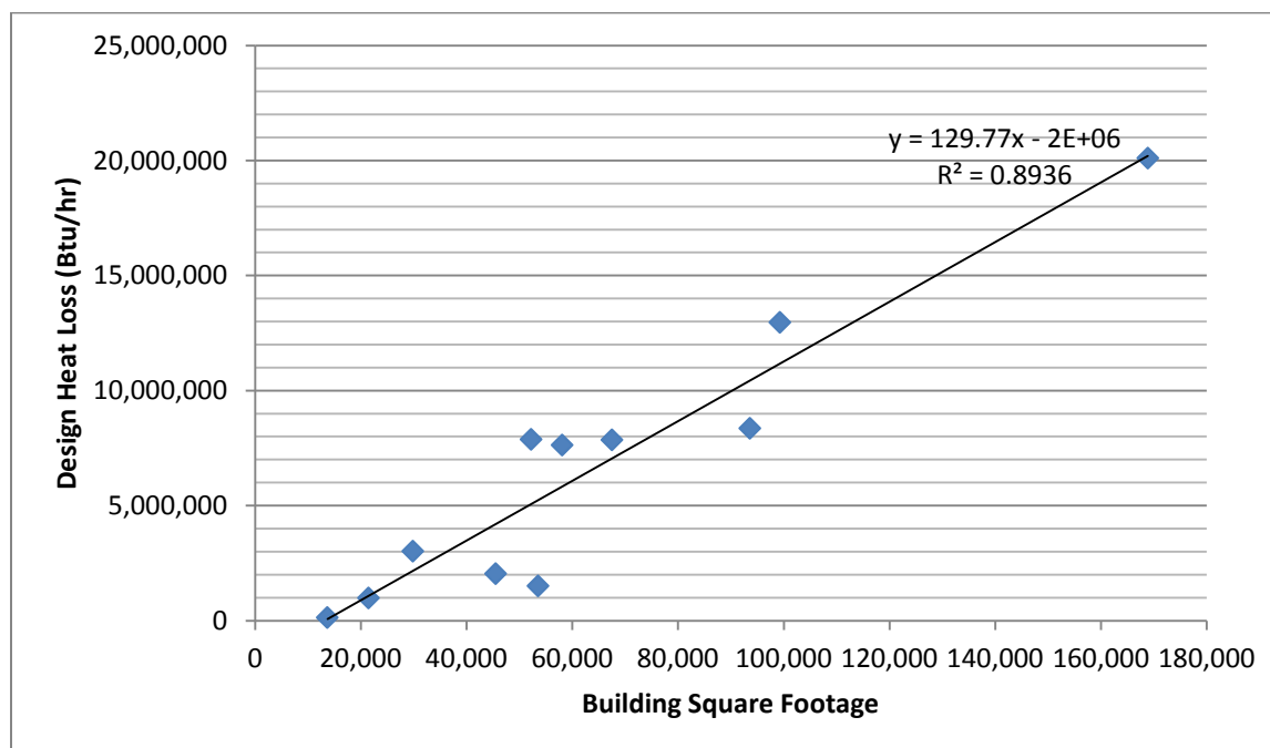
Figure 83: Design Heat Loss vs. Square Feet in Zone 6 Schools
