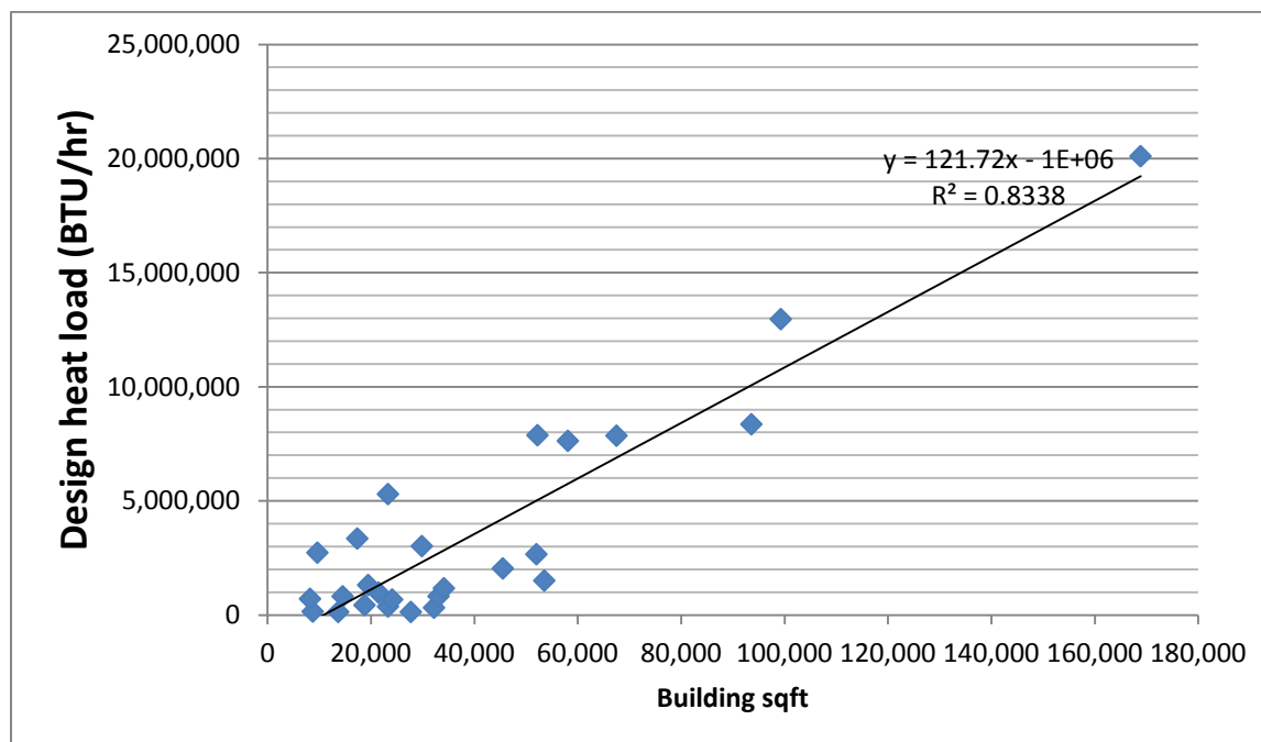
Figure 79: Zone 6 Design Heat Load for All Buildings
