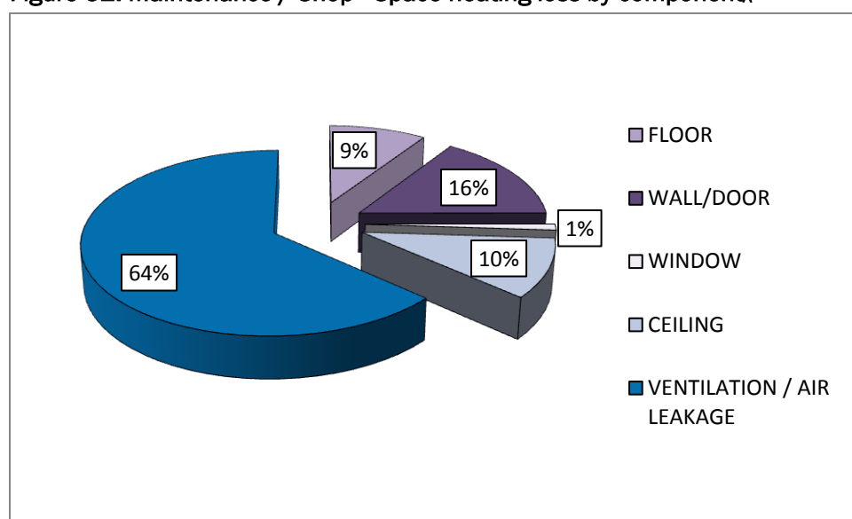
Figure 52: Maintenance / Shop - Space heating loss by component
