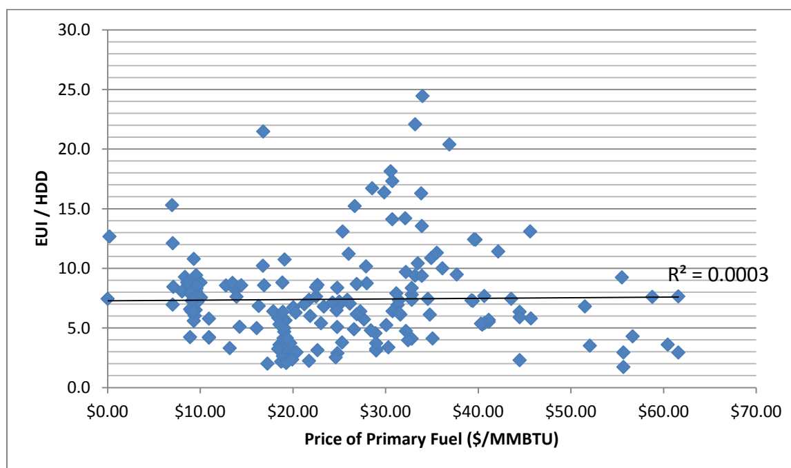
Figure AB: Thermal EUI/HDD vs. Primary Fuel Price for Schools
