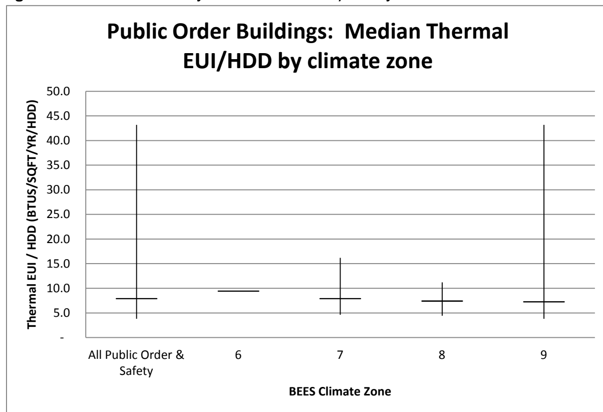
Figure 61: Public Order & Safety - Median Thermal EUI/HDD by Climate Zone a
