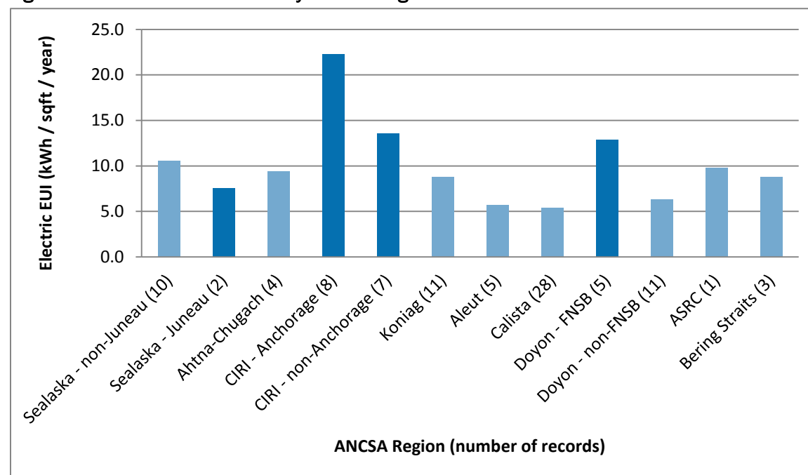
Figure 48: Offices - Electric EUI by ANCSA Region A+B
