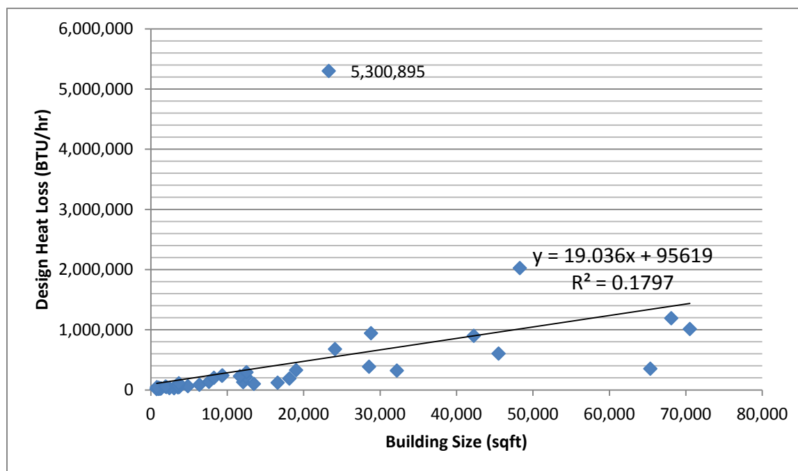
Figure 87: Design Heat Loss vs. Building Size in Maintenance/Shop Buildings
