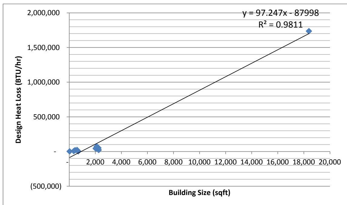
Figure 89: Design Heat Loss vs. Building Size in Washateria/Water Plants
