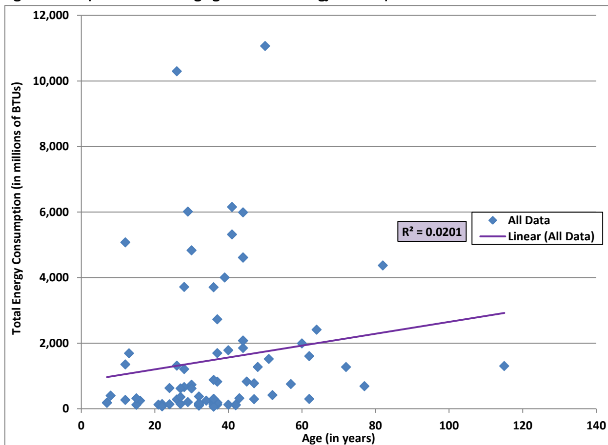
Figure N: Comparison of Building Age and Total Energy Consumption for Offices
