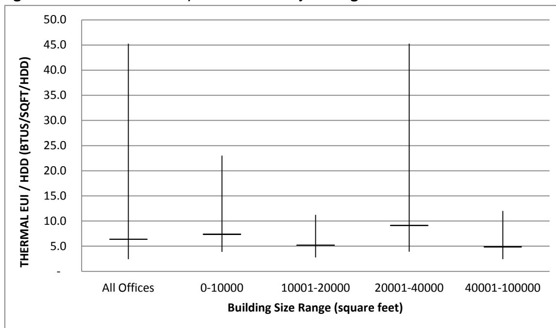
Figure 43: Median Thermal EUI/HDD for Offices by Building Size A
