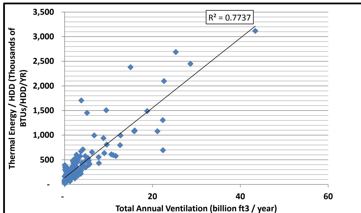
Figure 34: Schools: Annual thermal energy / HDD vs. Total Annual Ventilation
