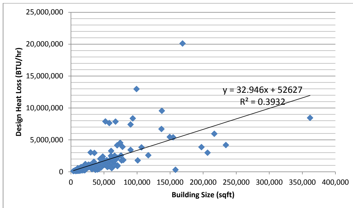
Figure 82: Design Heat Loss vs. Building Size for All Schools
