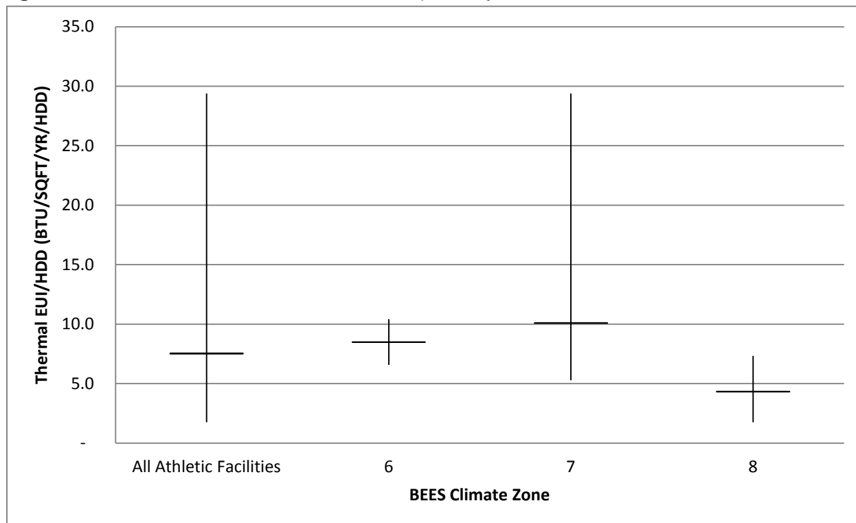
Figure 75: Athletic Facilities - Median thermal EUI/HDD by climate zone a
