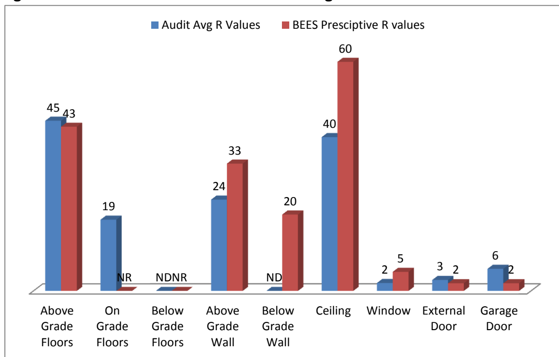
Figure 21: Zone 9 R-Values - BEES vs. Audited Buildings A
