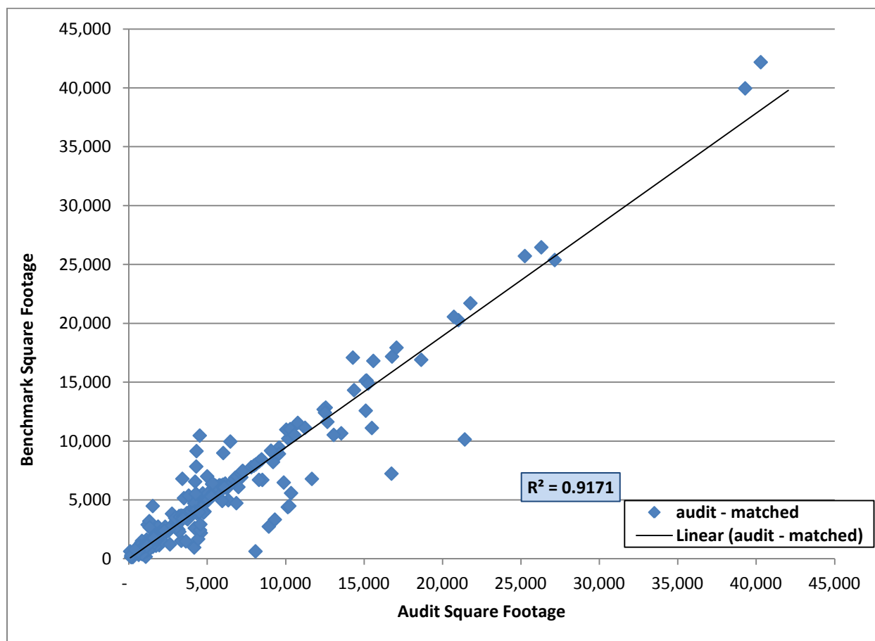
Figure K: Comparison of Benchmark and AHFC Audit Building Sizes
