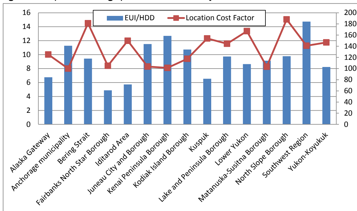
Figure AE: EUI/HDD vs. Geographic Area Cost Factor by School District
