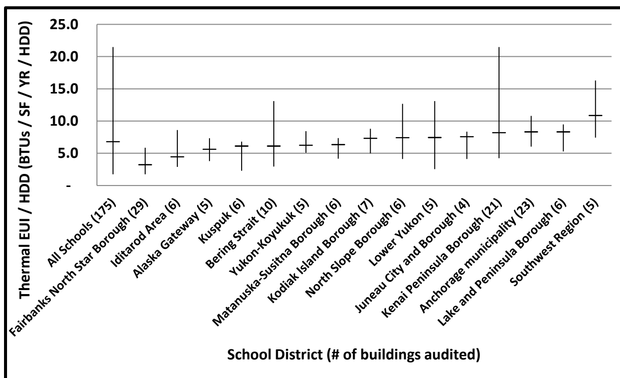
Figure 31: Median Thermal EUI/HDD by School District a
