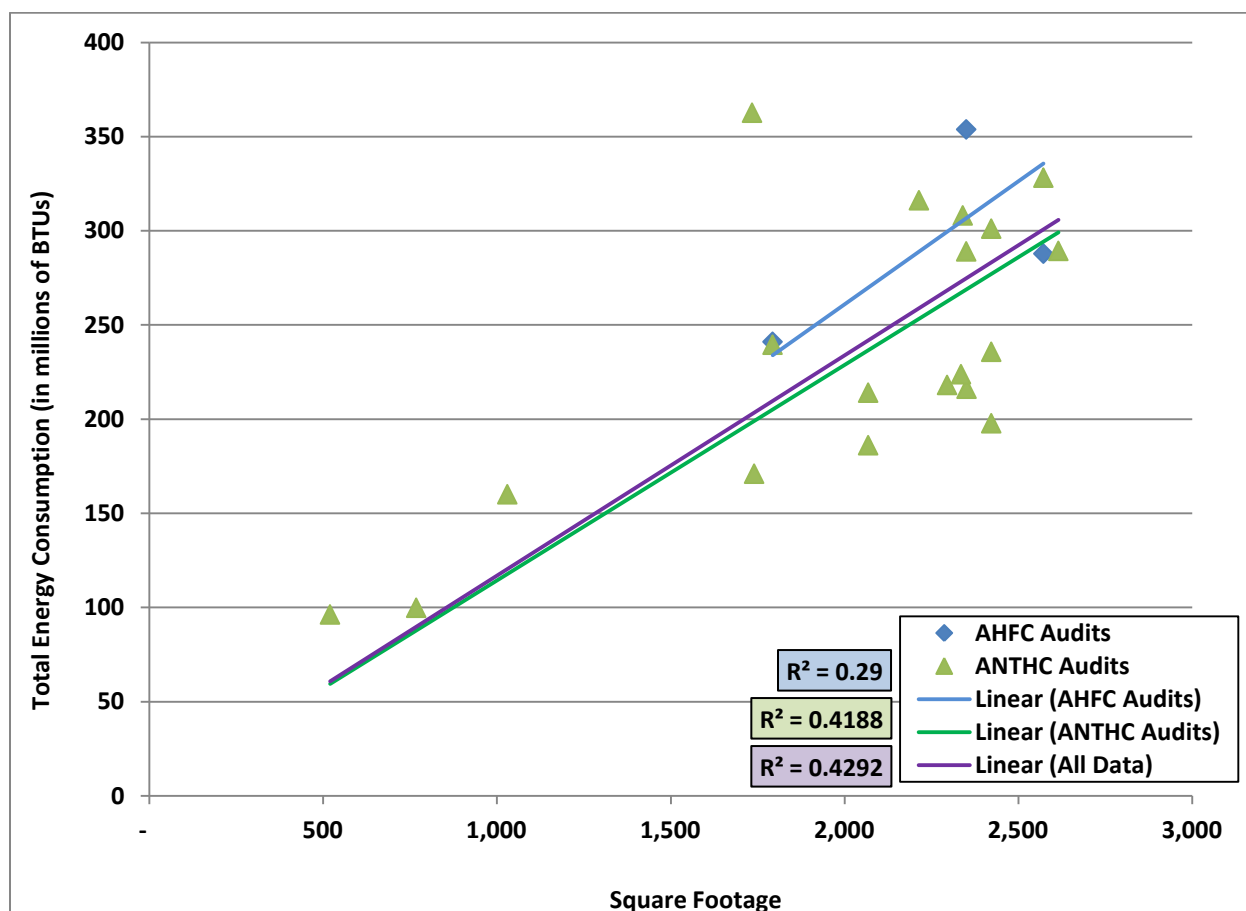
Figure H: Comparison of Health Clinic AHFC and ANTHC audit Data
