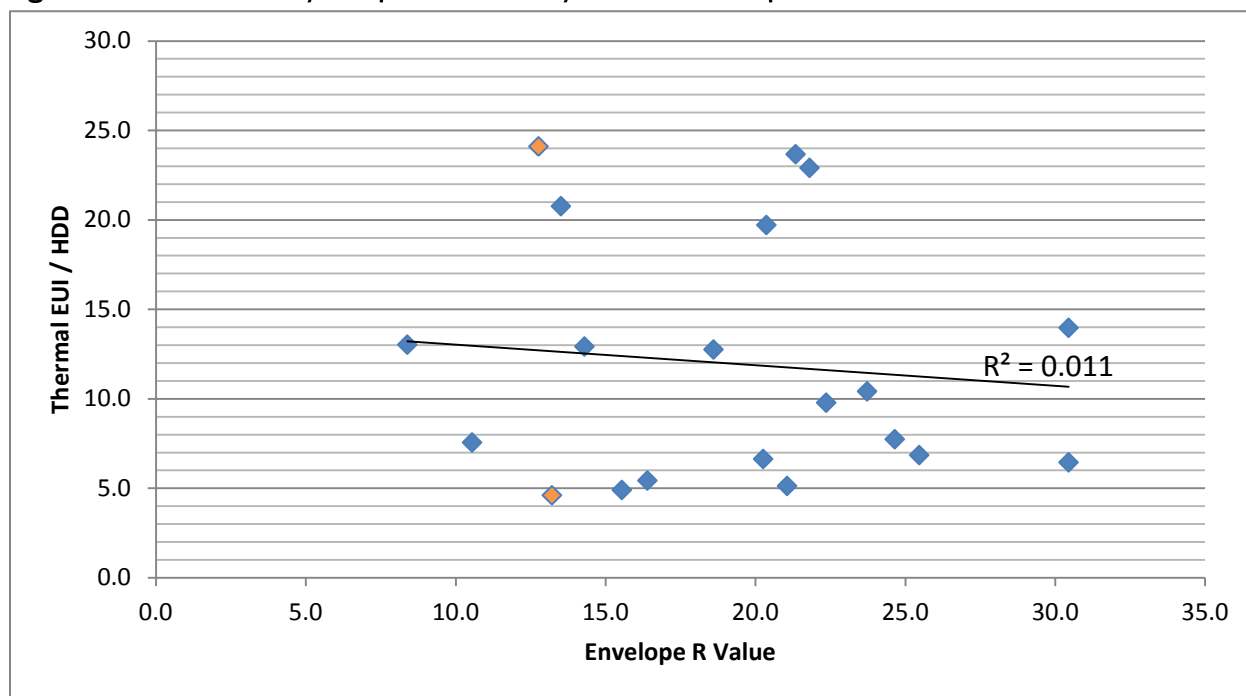
Figure 53: Maintenance / Shop - Thermal EUI/HDD vs. Envelope R-value
