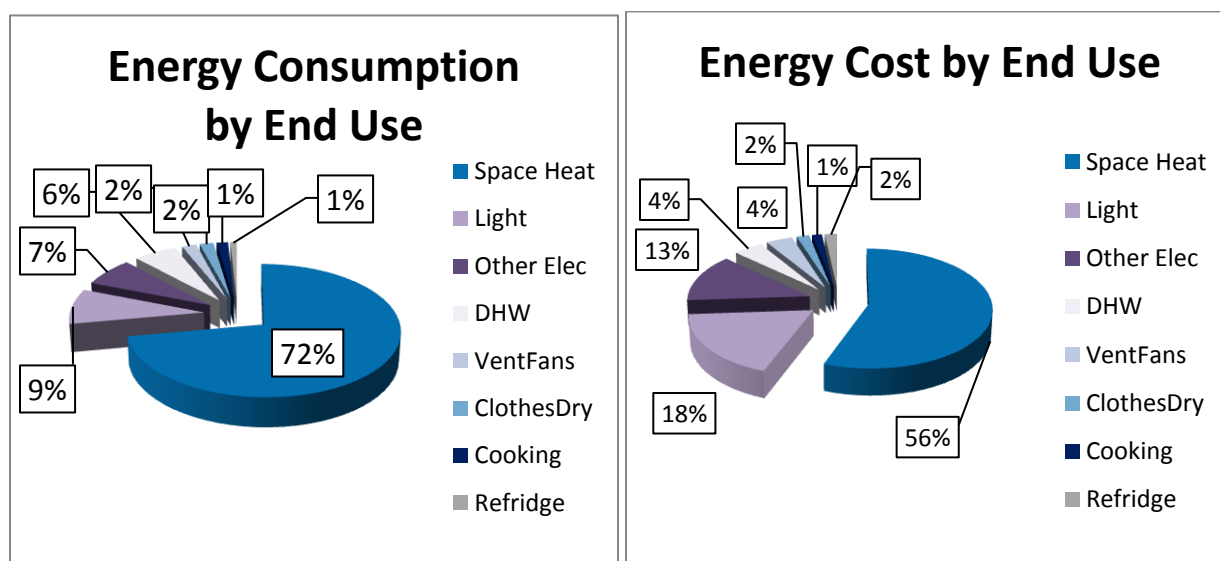
Figure 9: Energy Consumption and Cost by End Use
