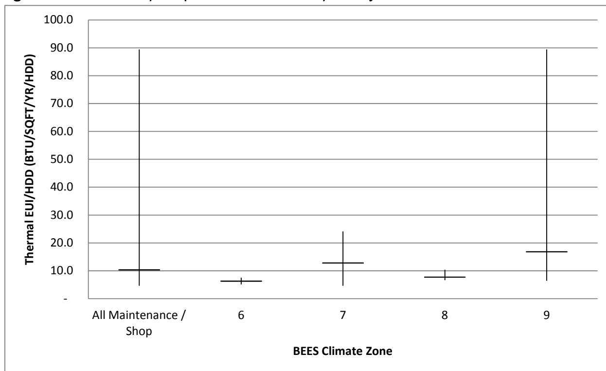
Figure 55: Maintenance / Shop - Median Thermal EUI/HDD by Climate Zone A
