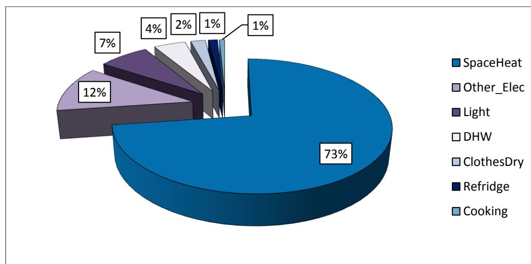
Figure 70: Health Clinic - Energy Consumption by End Use A
