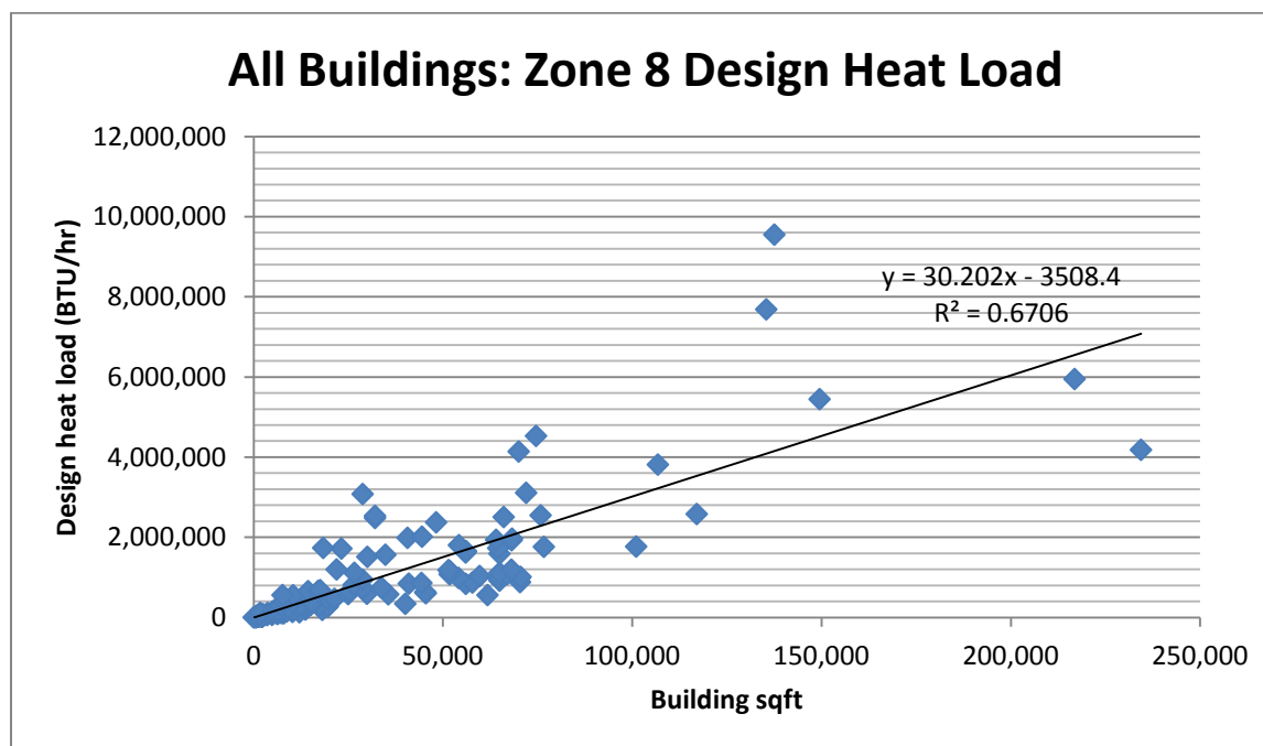
Figure 81: Zone 8 Design Heat Load for All Buildings
