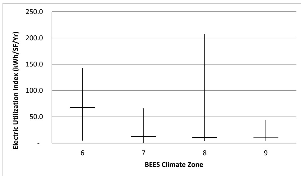
Figure 58: Maintenance / Shop - Median & Range Electric EUI by Climate Zone A+B
