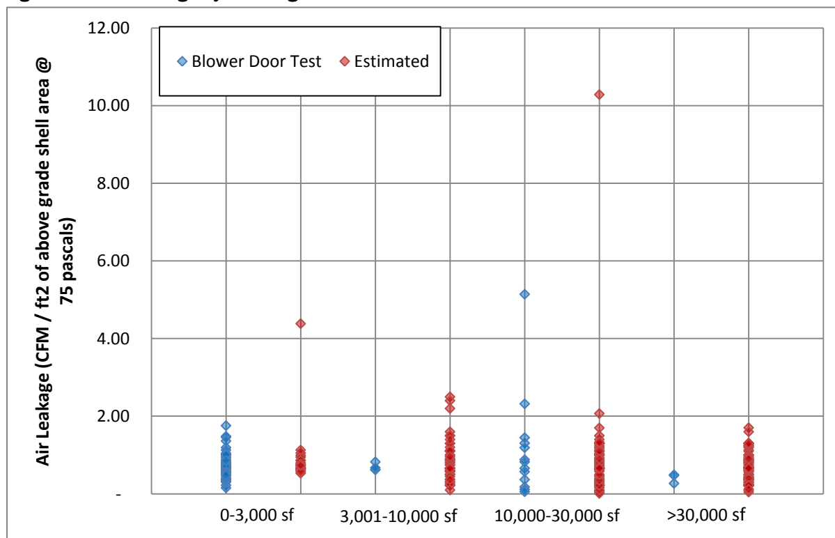
Figure 17: Air Leakage by Building Size Plot - Blower Door vs. Estimated A
