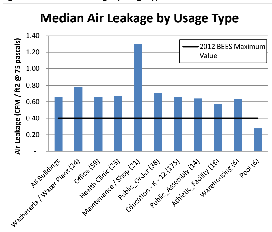
Figure 54: Median Air Leakage by Usage Type a
