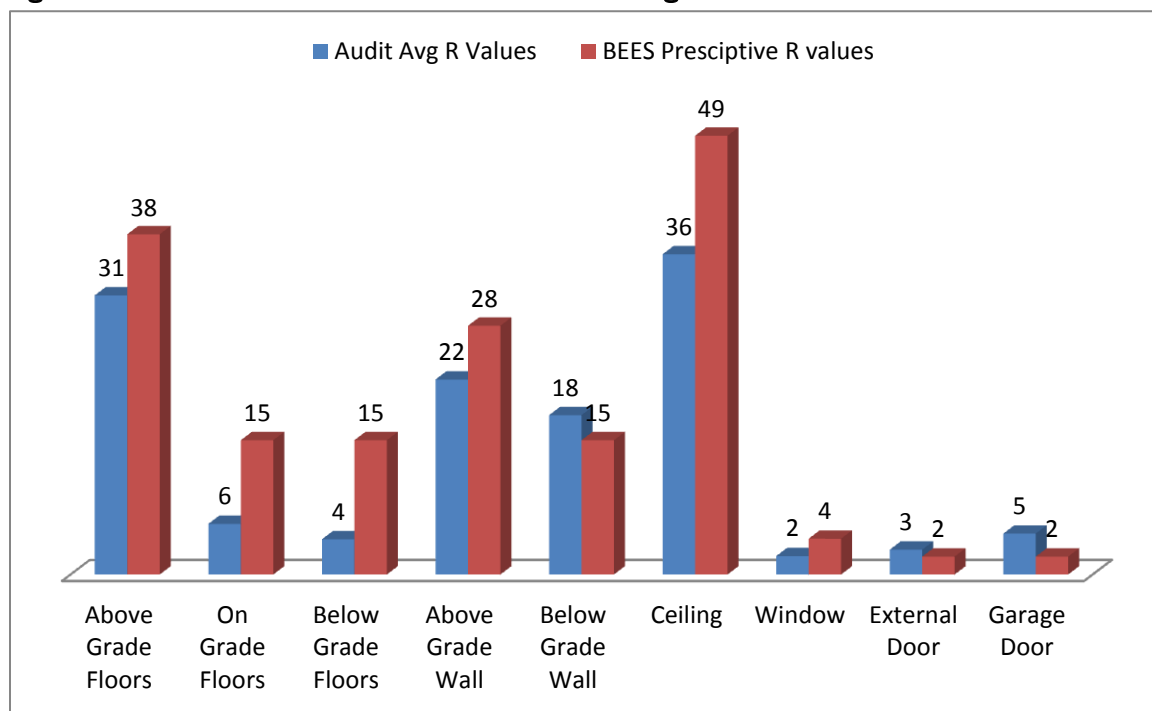
Figure 20: Zone 8 R-values - BEES vs. Audited Buildings a
