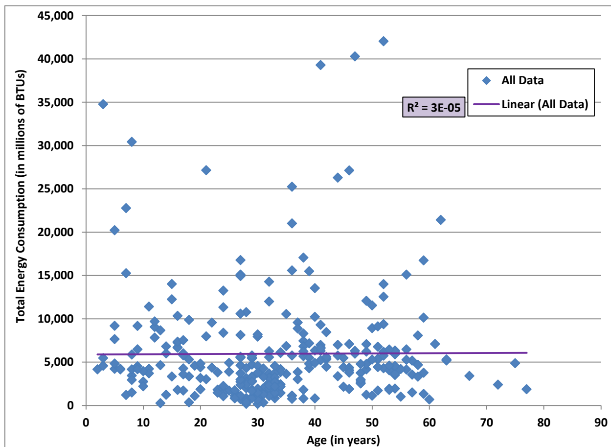
Figure M: Comparison of Building Age and Total Energy Consumption for Schools
