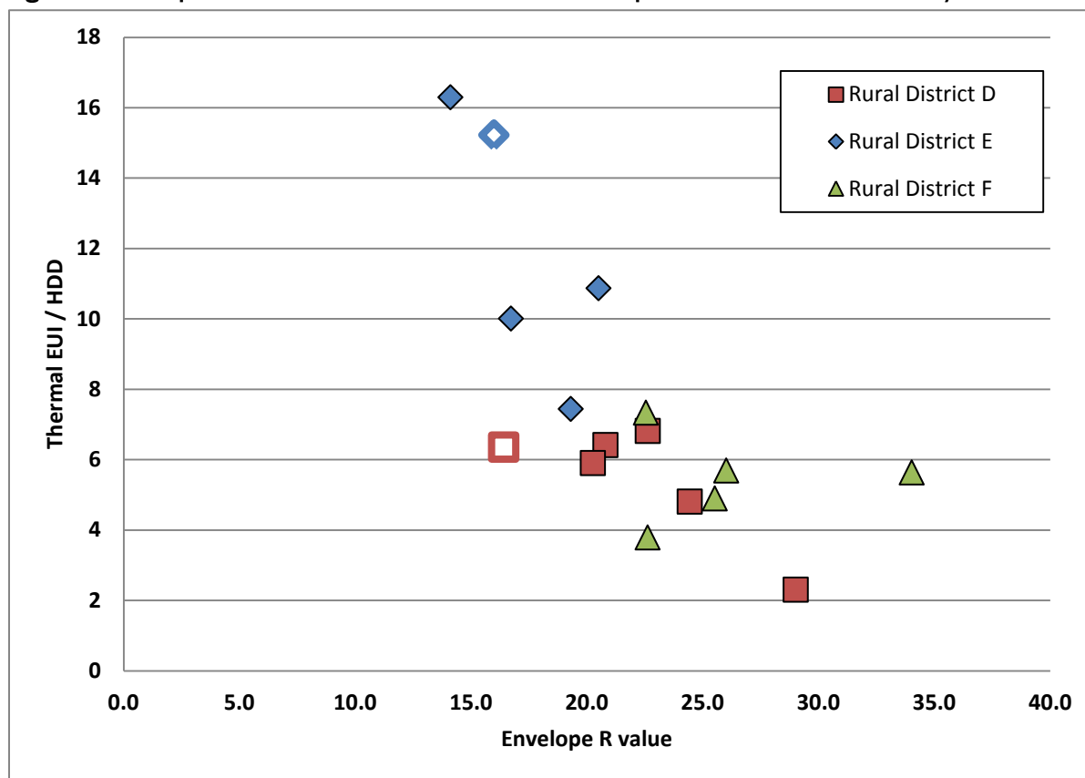
Figure 36: Comparison of Rural School Districts: Envelope R-values vs. Thermal EUI/HDD A
