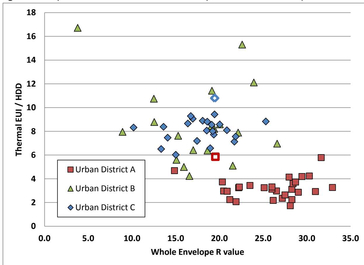
Figure 35: Comparison of Urban School Districts - Envelope R-value vs. Thermal EUI/HDD A
