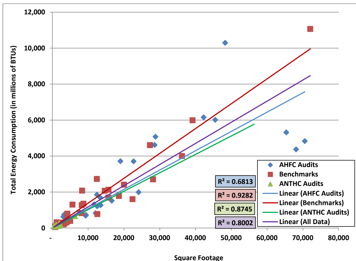
Figure C: Comparison of Office Benchmark, AHFC Audit, and ANTHC Audit Data
