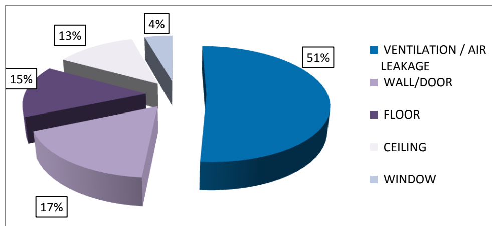
Figure 10: Space heat loss by component for all audited buildings a
