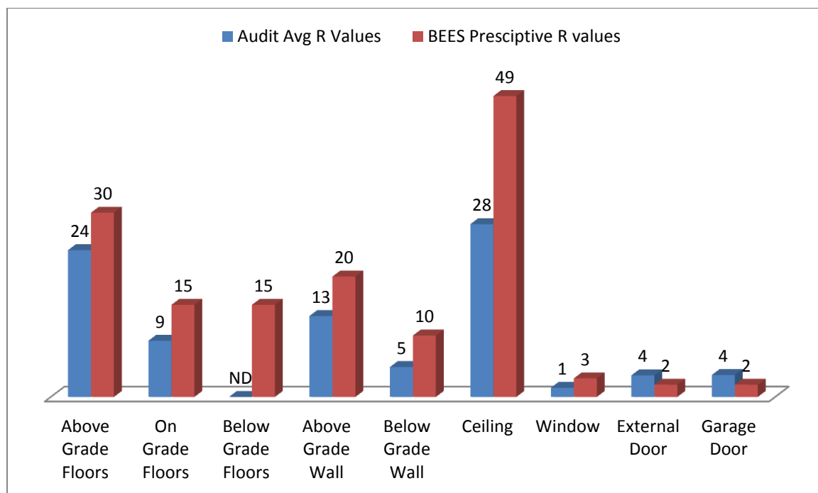
Figure 18: Zone 6 R-values - BEES vs. Audited Buildings A
