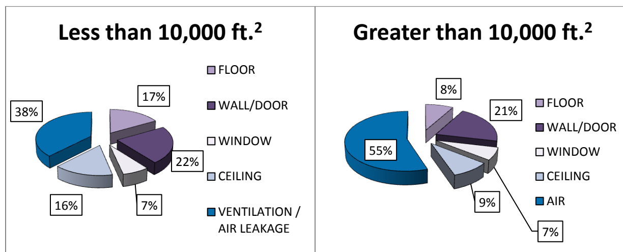
Figure 41: Offices by Size - Space Heating Loss by Component a
