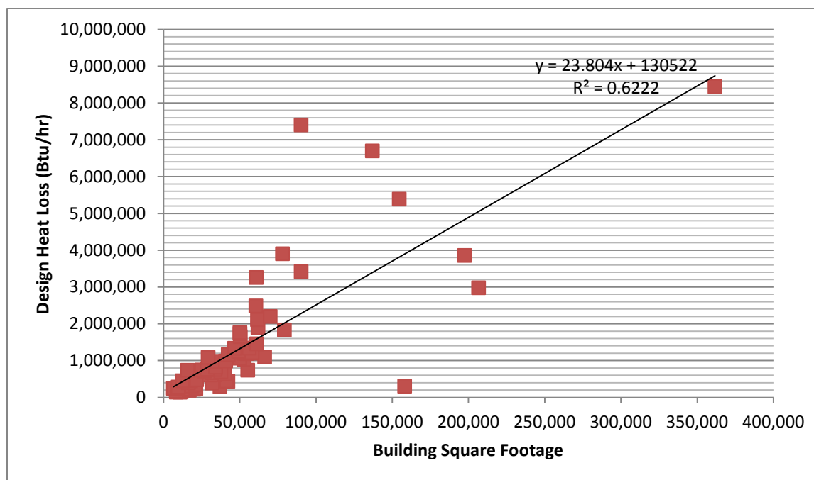
Figure 85: Design Heat Loss vs. Square Feet in Climate Zone 8 Schools
