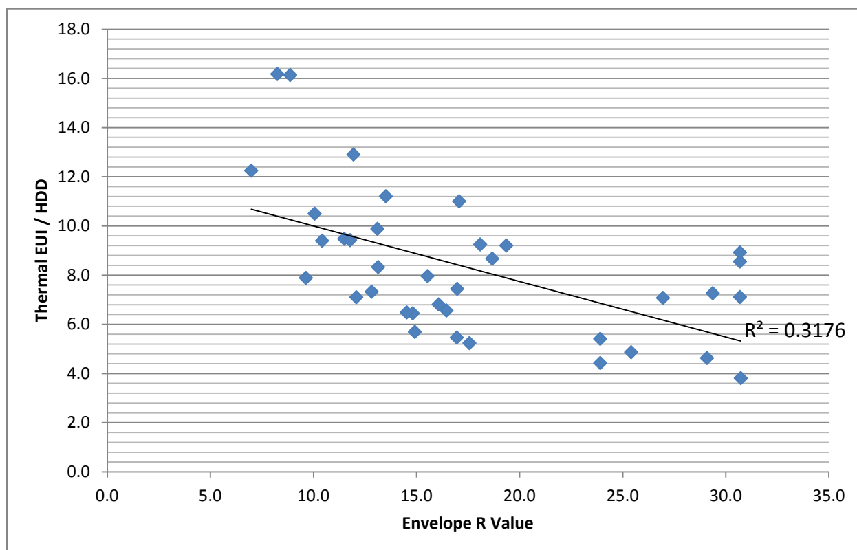
Figure 62: Public Order & Safety - Thermal EUI/HDD vs. Envelope R-value A
