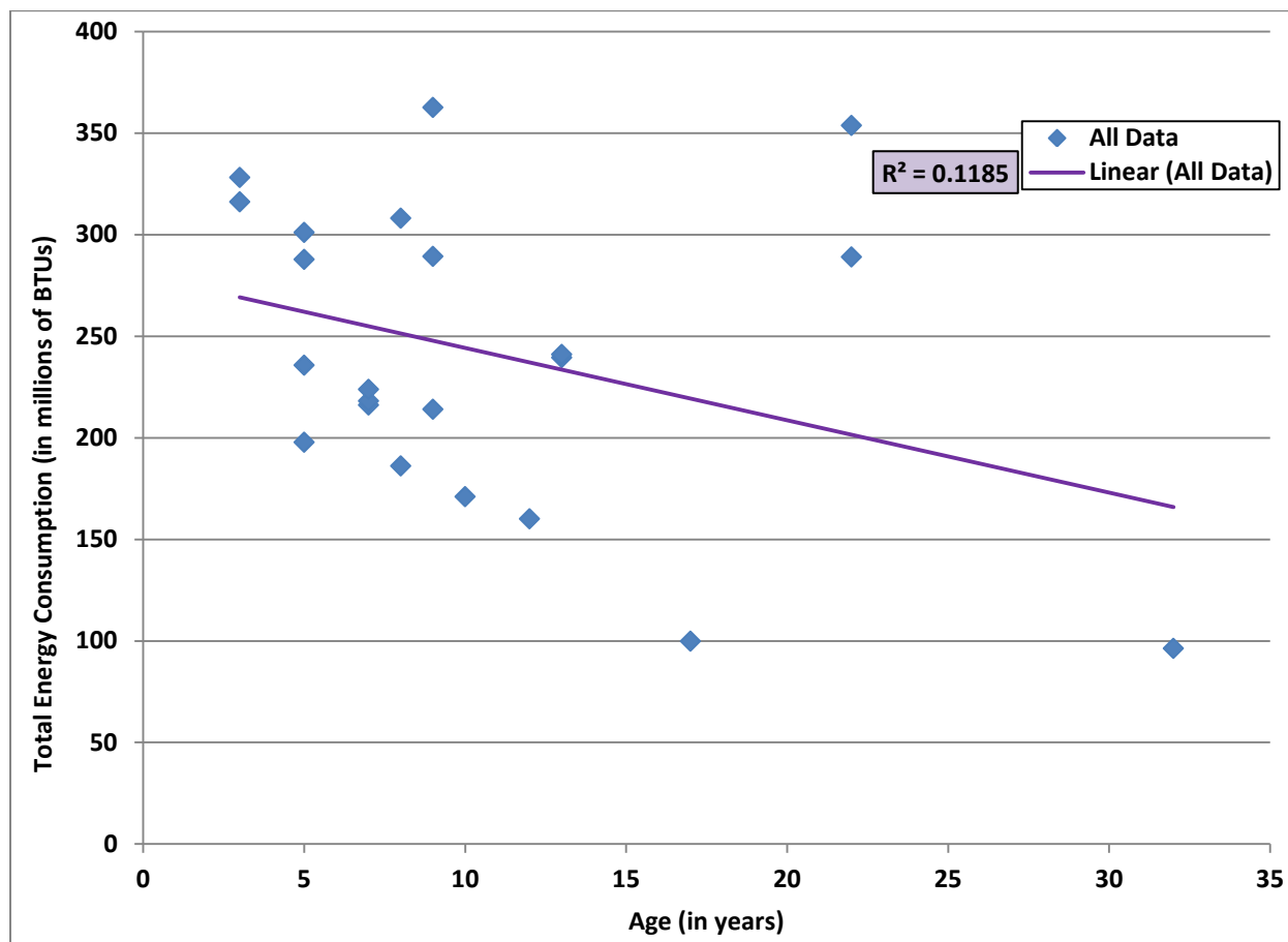
Figure P: Comparison of Building Age and Total Energy Consumption for Health Clinics
