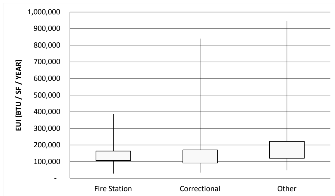
Figure 67: Public Order & Safety - EUI by Sub-type A+B
