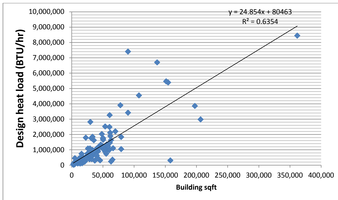
Figure 80: Zone 7 Design Heat Load for All Buildings
