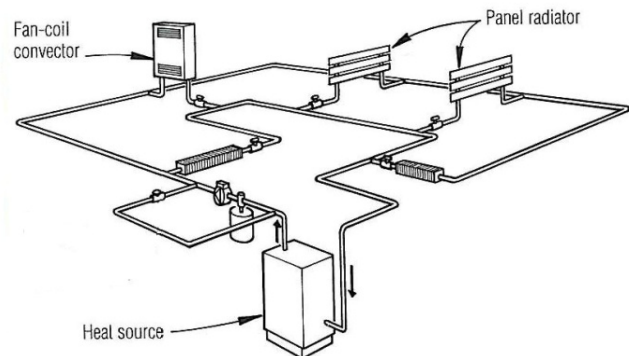
A two-pipe system has separate supply and return pipes. Image from Journal of Light Construction, 2005.
